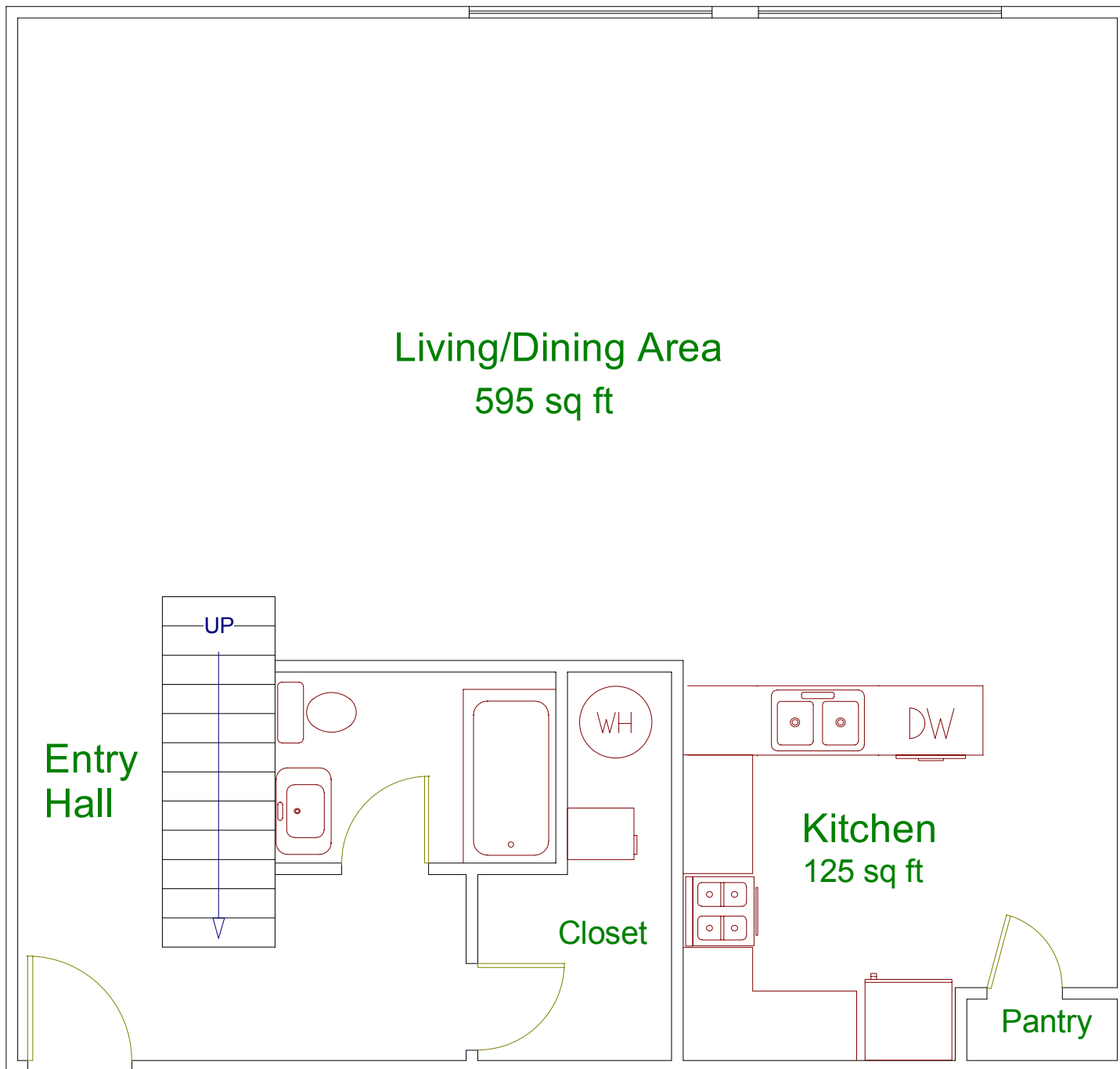
1 Bedroom Loft Apartment Main Level Plan
